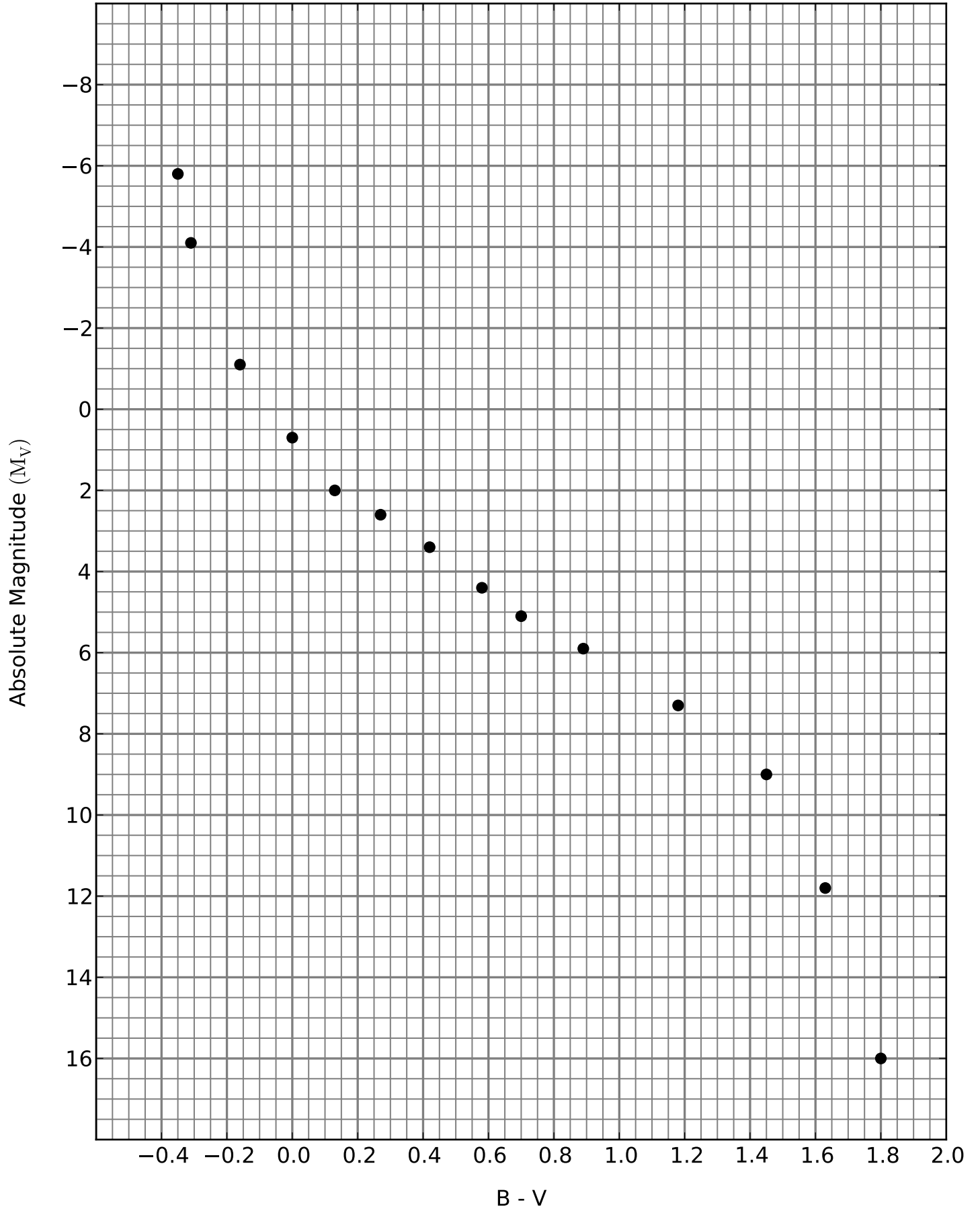
HR Diagram of Calibration Stars
